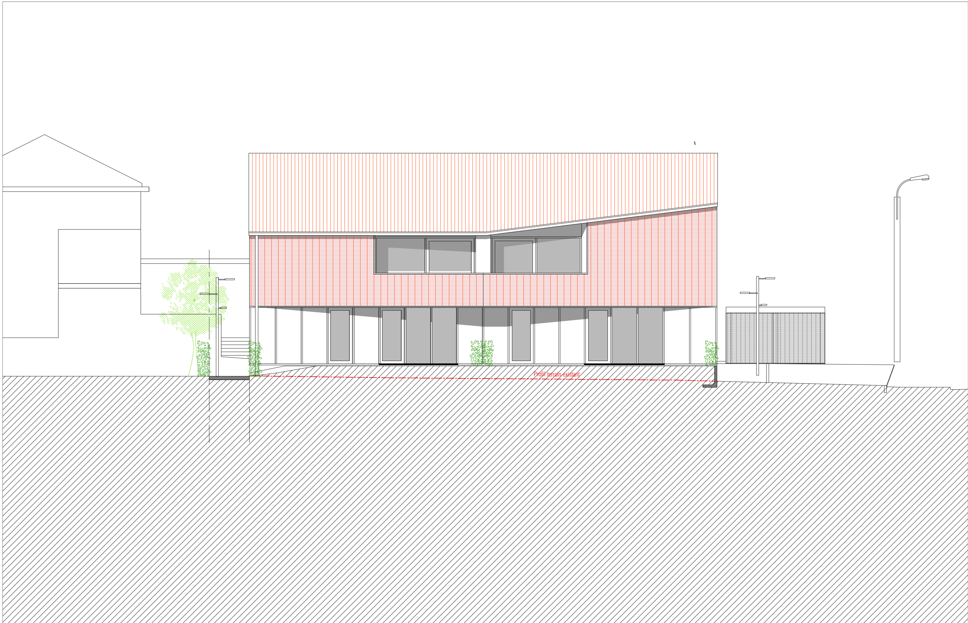
BLOC B FACADE JARDIN
